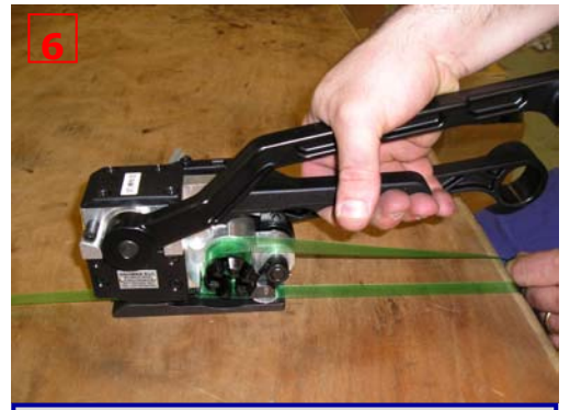
CUTTING STRAP – OPEN TOOL
